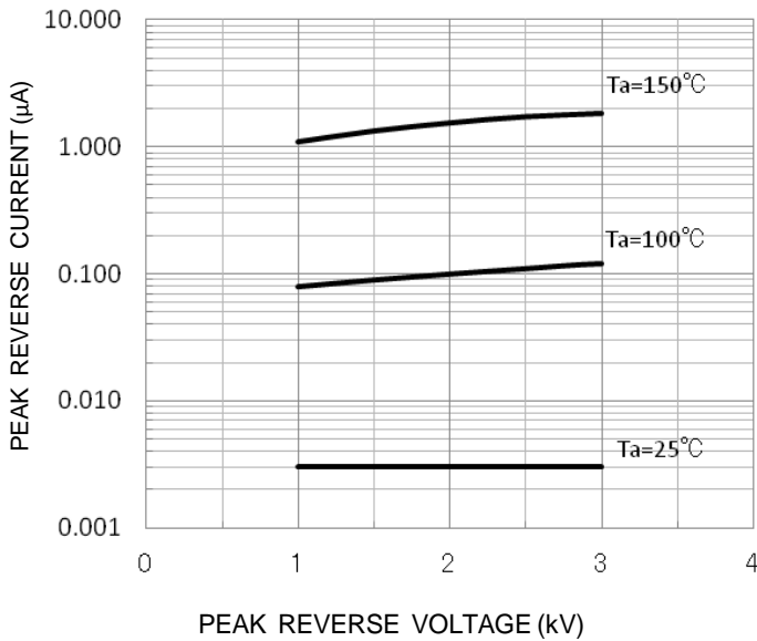
Typical Reverse Current characteristic ( I_r : 0.001\mu\text{A} \sim 10\mu\text{A} )
